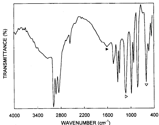
Figure 3. FT-IR spectrum of Titanium isopropoxide, (\text{Ti}(\text{OR})_4) .
