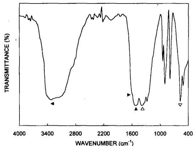
Figure 2. FT-IR spectrum of Lead Acetate Trihydrate, ( \text{Pb}(\text{Ac})_2 \cdot 3\text{H}_2\text{O} ).
