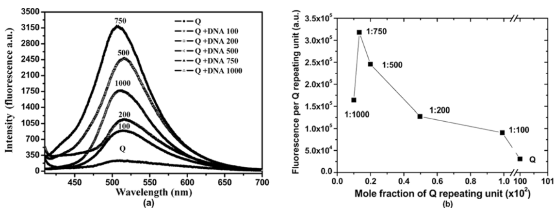
Figure 4. Fluorescence spectra (a) of DNA-Q complexes (molar ratio of the repeating unit) and (b) dependence of fluorescence intensity per Q repeating unit on its mole fraction in the mixtures.
