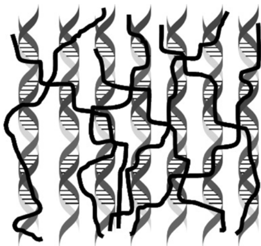
Figure 1. Mixture of DNA and Polymer Q.
